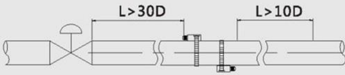
Install after valves
