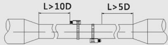
Install on diameter-reduced pipe
