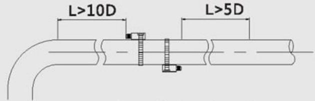
Install after the elbow
