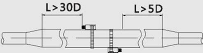
Install on diameter-expanded pipe
